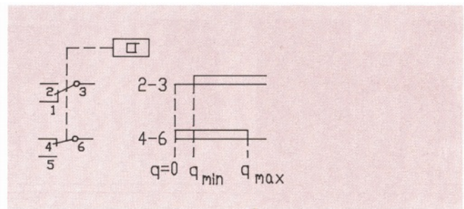
Type TIVG ...F for flange connection
